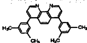
Structural formula 5:
